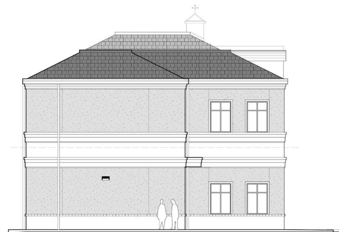
EAST ELEVATION (facing side yard) SCALE: 1 : 100
